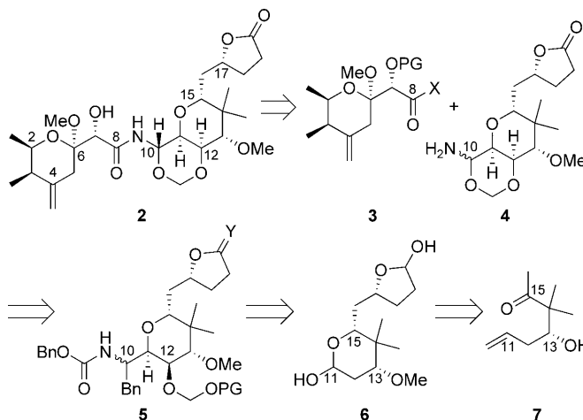
Scheme 2. Retrosynthetic analysis of theopederin D. Bn = benzyl, PG = protecting group.
