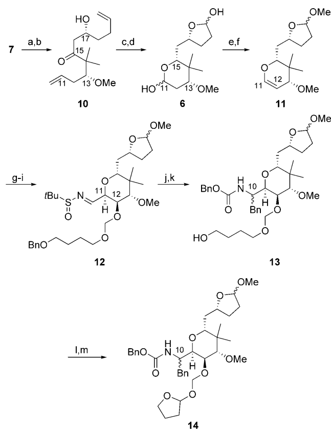
Scheme 4. Synthesis of the cyclization substrate 14 . Reagents and conditions: a) MeOTf, DTBP, CH 2 Cl 2 , 88%; b) (+)-Ipc 2 BCl, Et 3 N, Et 2 O; then 5-pentenal, 65%, d.r. 10:1; c) Et 2 BOMe, THF; then NaBH 4 , MeOH, 77%; d) OsO 4 , NaIO 4 , THF, H 2 O, 82%; e) PPTS, MeOH; f) TFAA, iPr 2 NEt, CH 2 Cl 2 , 92% (over 2 steps); g) DMDO, acetone; then trivinylalane, CH 2 Cl 2 , 100%; h) BBMCl, iPr 2 NEt, CH 2 Cl 2 , 77%; i) O 3 , CH 2 Cl 2 , -78 °C; then (R)-tBuS(O)NH 2 , Ti(OiPr) 4 , CH 2 Cl 2 , 50%, 62% (based on recovered aldehyde); j) BnMgCl, THF, 65%; k) HCl, MeOH, 80%; l) H 2 , Pd/C, MeOH; then CbzCl, Et 3 N, CH 2 Cl 2 , 70%; m) PhI(OAc) 2 , hν, cyclohexane, 80%. BBM = benzyloxybutoxymethyl; Cbz = benzyloxycarbonyl, DMDO = 2,2-dimethyldioxirane, Ipc 2 BCl = diisopinocampheyl chloroborane, PPTS = pyridinium para -toluenesulfonate, Tf = trifluoromethanesulfonyl, TFAA = trifluoroacetic anhydride.
