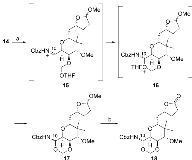
Scheme 5. Synthesis of the amido trioxadecalin 18 . Reagents and conditions: a) h\nu , NMQPF 6 , O 2 , NaOAc, Na 2 S 2 O 3 , toluene, DCE, 76 %; b) Jones reagent, acetone, 64 %. DCE = 1,2-dichloroethane.
