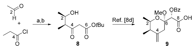
Scheme 3. Synthesis of benzoyl pederic acid 9 . Reagents and conditions: a) TMSQ, LiClO 4 , iPr 2 NEt, Et 2 O; b) LDA, tBuOAc, THF, 76% (over 2 steps). Bz = benzoyl, LDA = lithium diisopropylamide.
